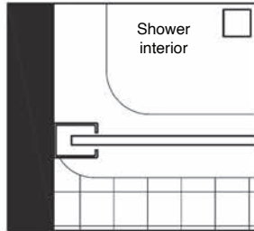
Installation on shower tray (C1)
